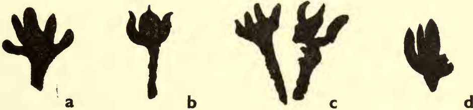
FIG. 15. Pseudovoltzia liebeana (Geinitz) Florin. Cone scales. (a), Marl Slate, Kimberley. British Museum (Natural History), no. V.35128; (b, c), Hilton Plant Beds, Hilton. Geological Survey, nos. 19073, 19074; (d), Hilton Plant Beds, Hilton. British Museum (Natural History), no. V.35119. All \times 1.6 .
